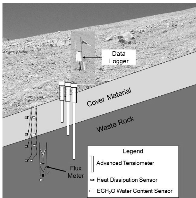
Figure 2 Cross-section of monitoring nest installation
