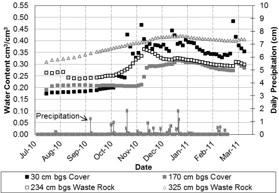
Figure 8 Water content and precipitation at NFU
