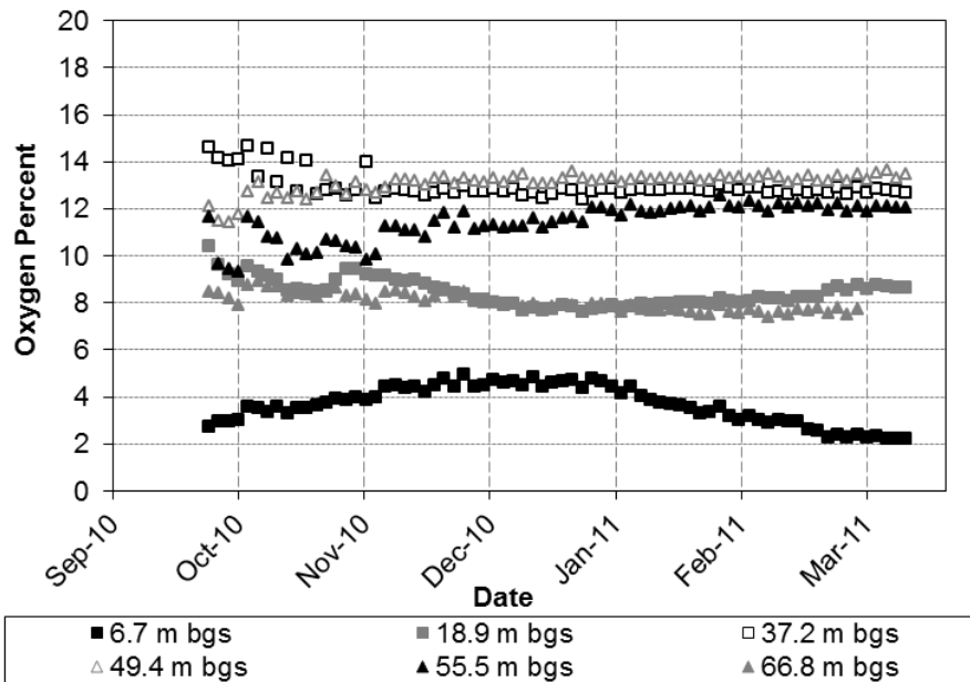
Figure 7 SICU geochemical borehole oxygen content
