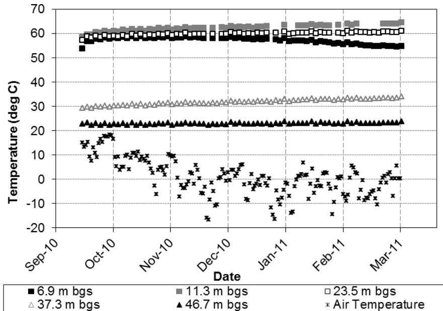
Figure 10 NFU geochemical borehole air and soil temperature
