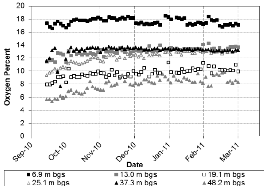
Figure 11 NFU geochemical borehole oxygen content
