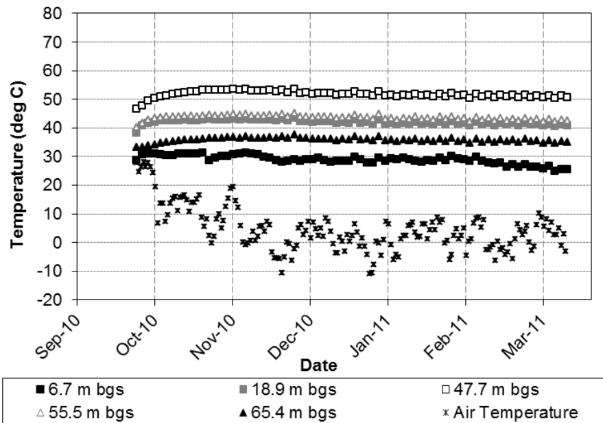
Figure 6 SICU geochemical borehole air and soil temperature
