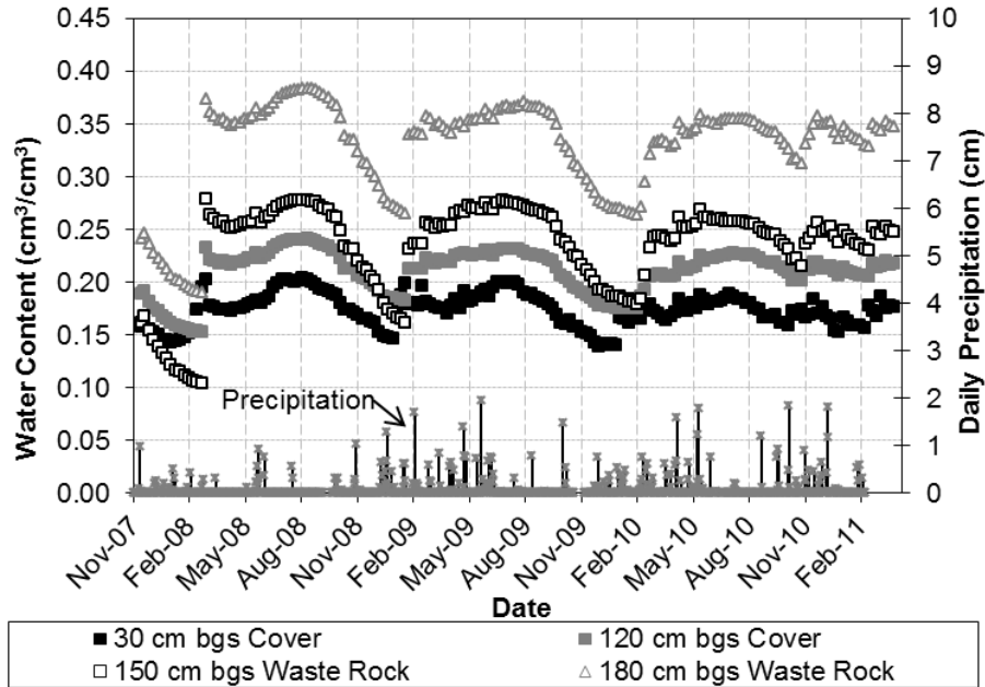
Figure 4 Water content and precipitation at SICT
